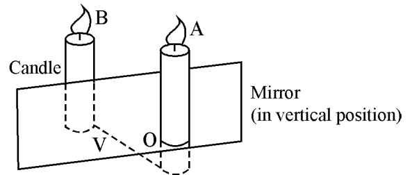
Fig. : Position of image
