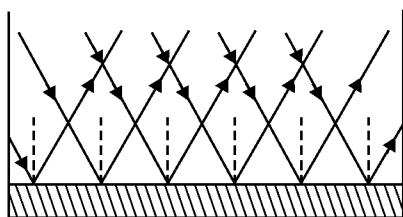
Fig. : Regular reflection
