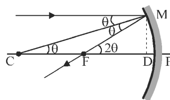
Fig. : Concave spherical mirror
